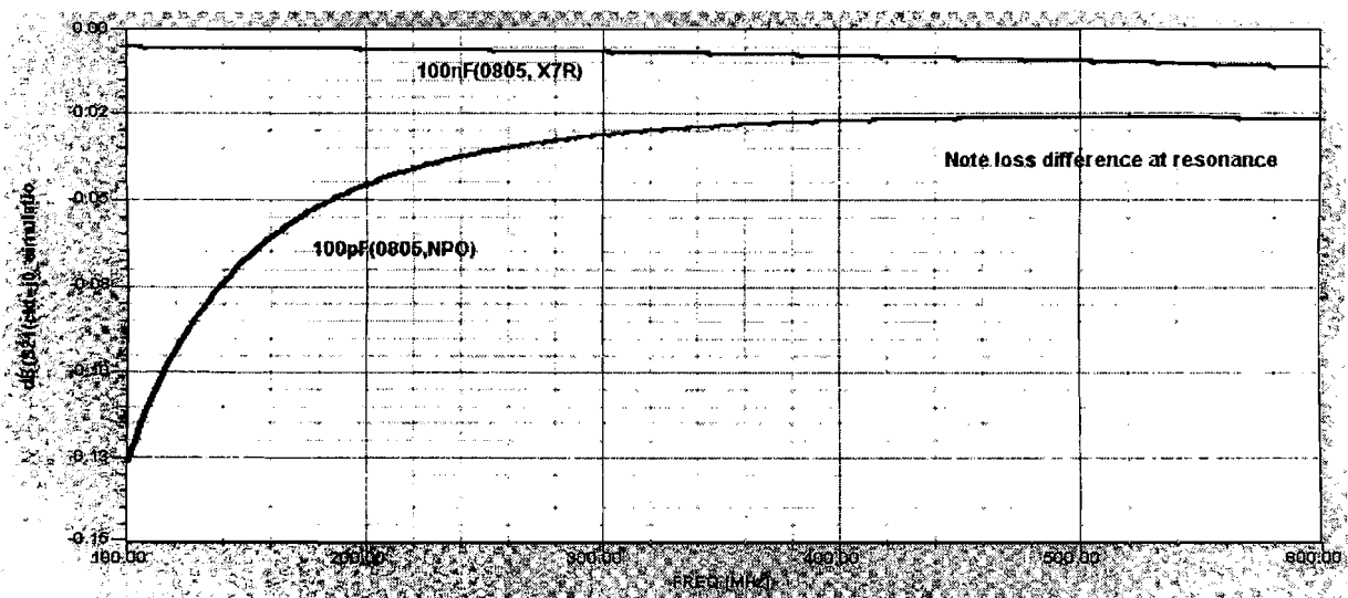
Figure 22: Comparison of 100n,X7R and 100pF, NPO capacitor insertion loss.
