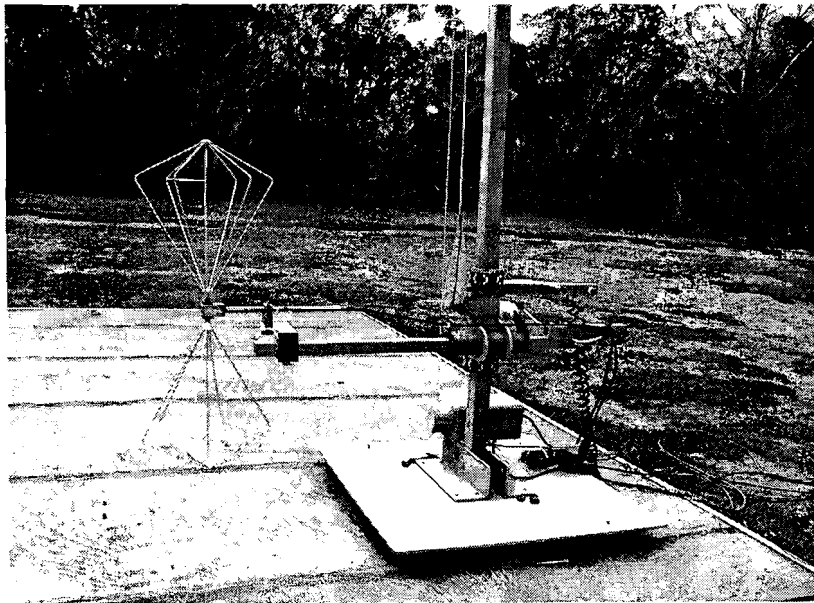
Figure 24 – A broadband antenna used for testing to 230MHz.
