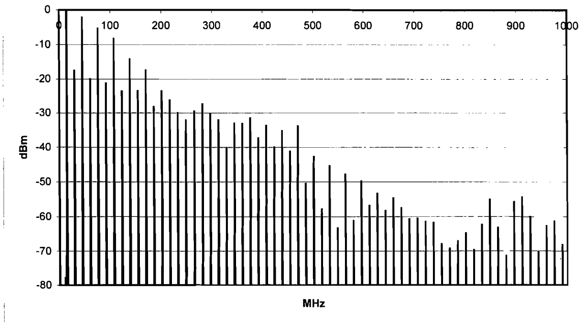
Figure 7 - 16MHz into AC MOS buffer, filtered by 10R and 100pF RC Filter (50R system)
