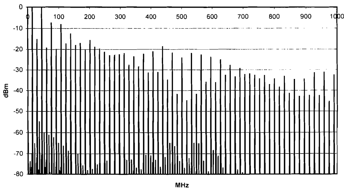
Figure 6 - 16MHz into AC MOS buffer (50R system)
