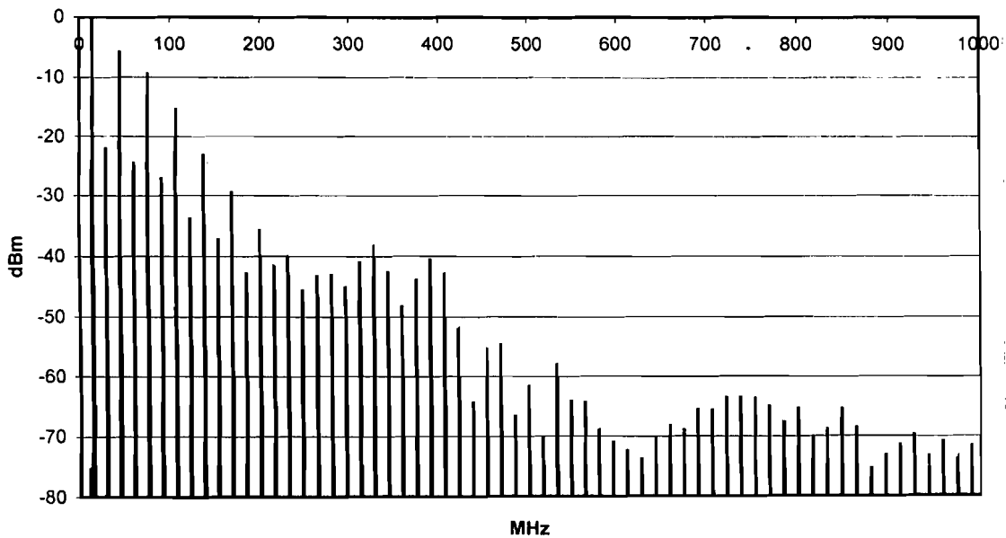
Figure 9- 16MHz into AC MOS buffer, filtered by BLM41 bead and 100pF cap (50R system)
