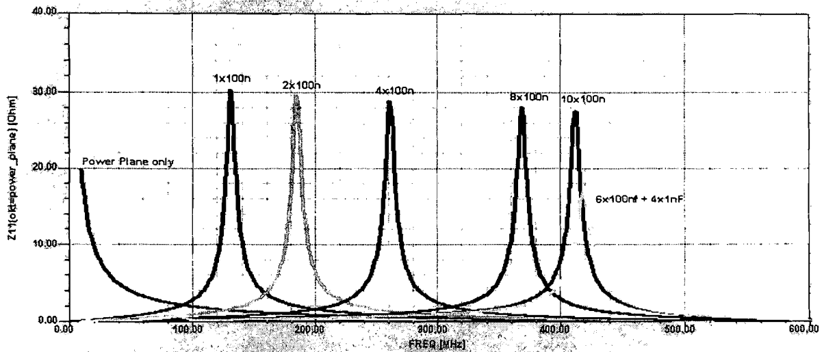
Figure 15: Simulation of power plane impedance with bypass capacitor combinations
