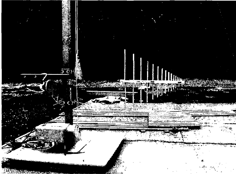
Figure 25 – Log Periodic antenna used for testing 230MHz-1GHz (Equipment courtesy of EMC Technologies Pty Ltd)
