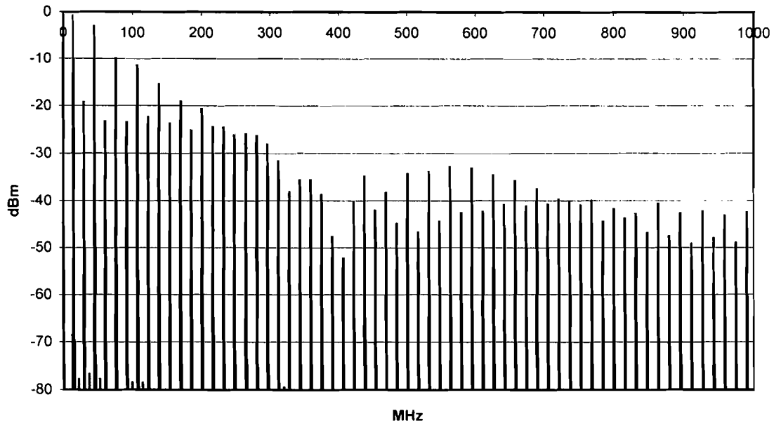
Figure 8 -16MHz into AC MOS buffer, filtered by BLM41 Ferrite Bead (50R system)
