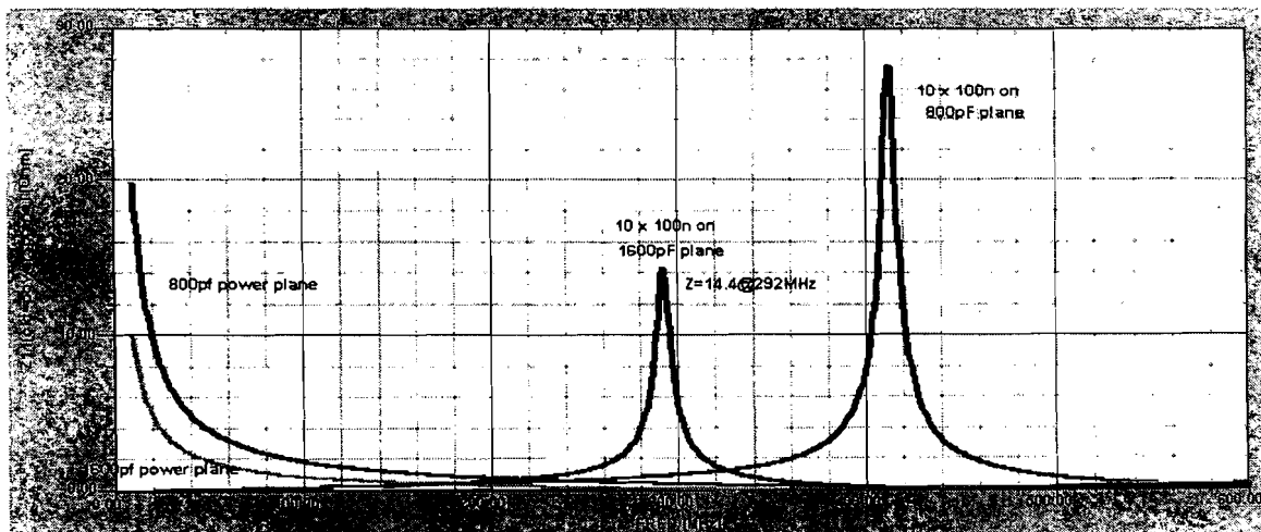
Figure 19: Comparison of two power plane core thicknesses
