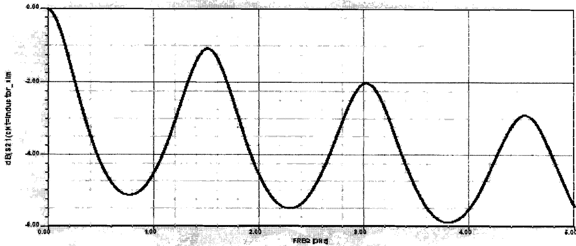
Simulated insertion loss plot of a track 0.2mm x60mm on 1.6mm FR4 PCB
