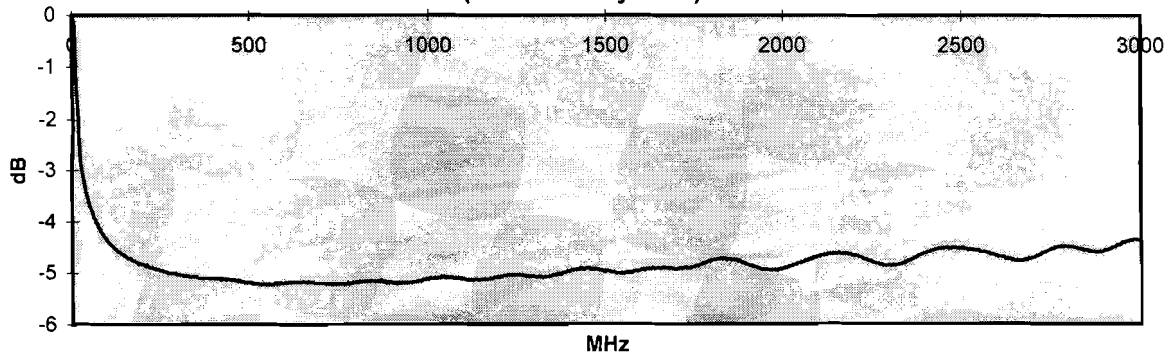
Figure 4 - BLM31A700 RF Bead measured transmission loss (in 50 ohm system)
