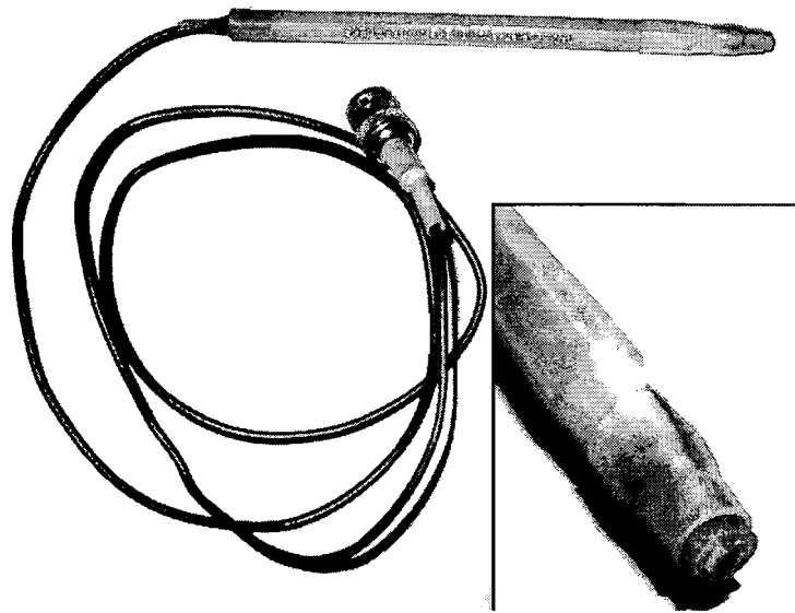
Figure 1 – A home made inductive probe.
