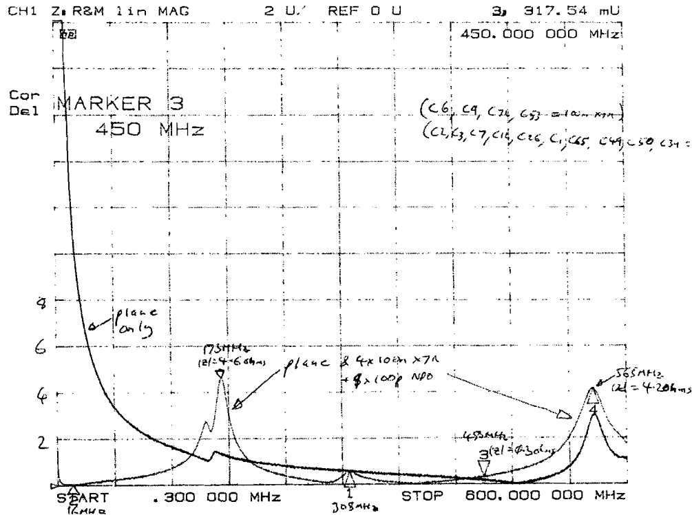
Figure 17: Network Analyser plot of modified plane impedance.
