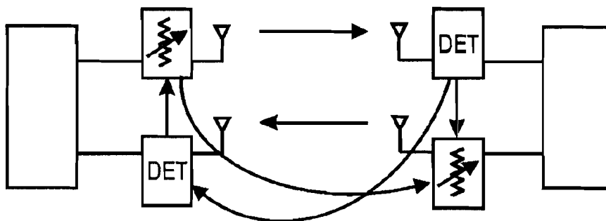
Figure 3 - Double Ended Power Control - Closed Loop
