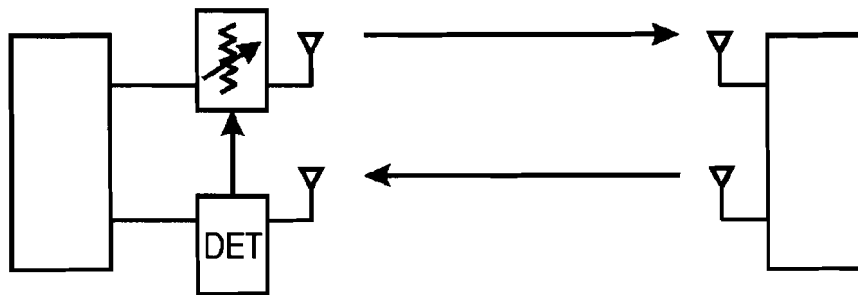
Figure 1 - Single Ended Power Control
