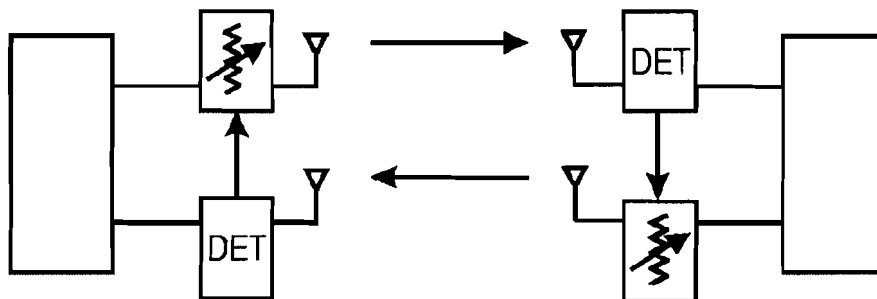
Figure 2 - Double ended Power Control - Open Loop
