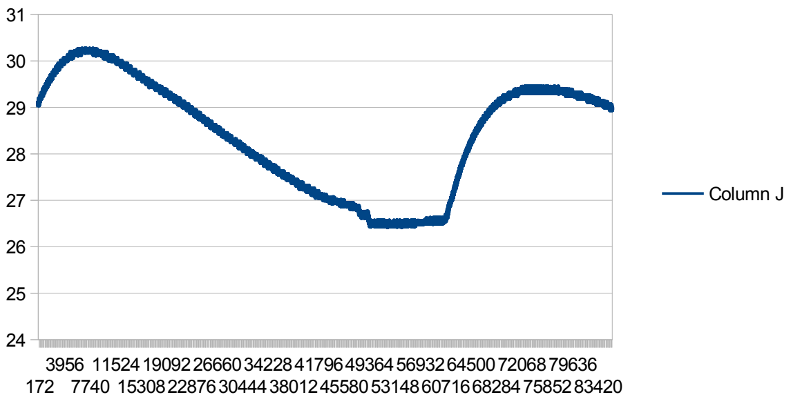
24 hour temperature RM3100 i2c interface board for GTJ run of 06-30-2020
