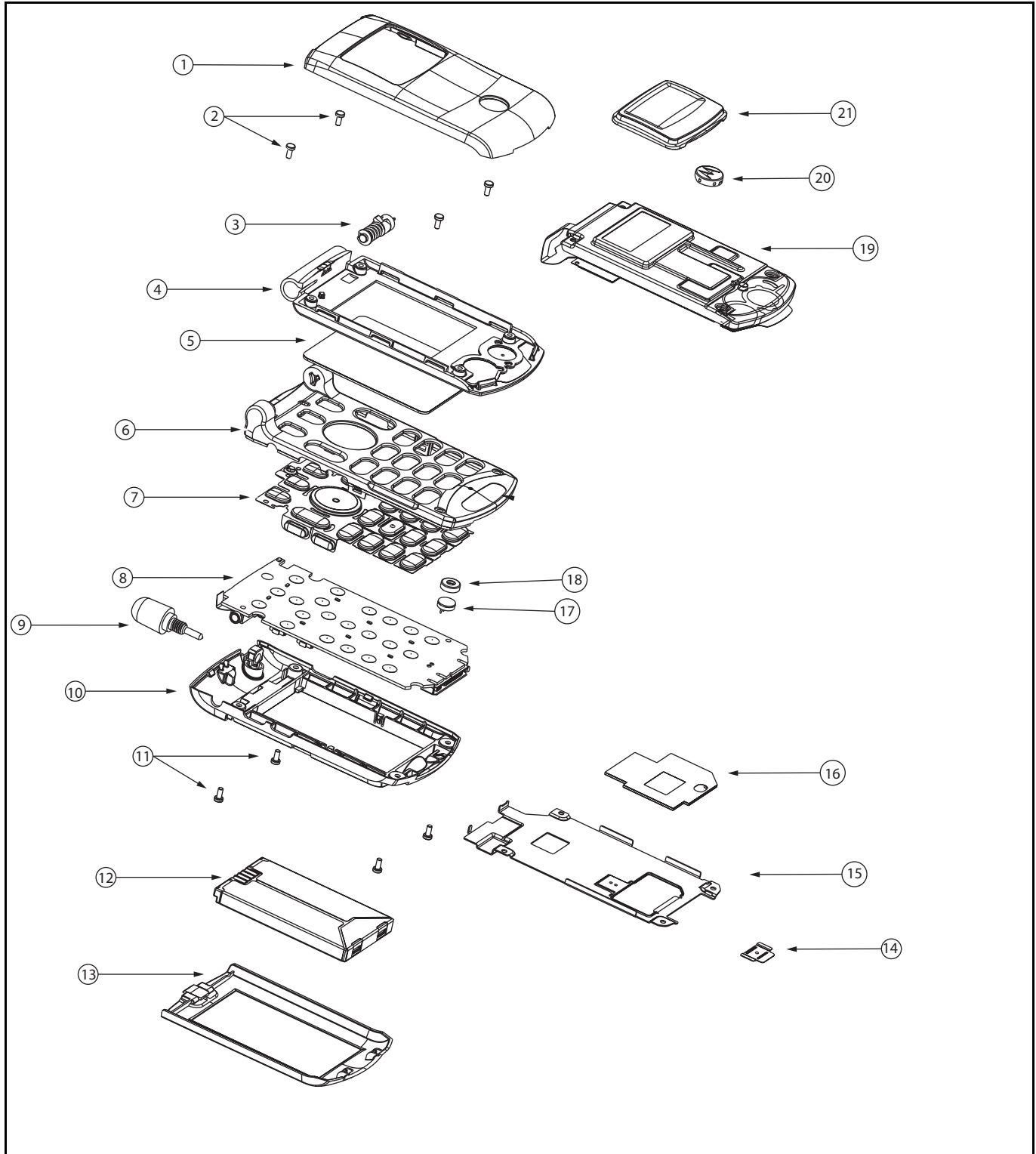
Figure 21. Exploded View
