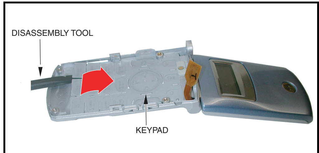
Figure 12. Removing the Keypad
