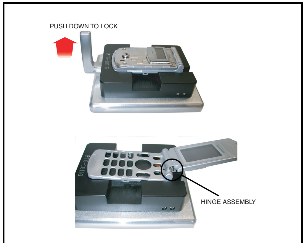
Figure 15. Removing the Flip Assembly From the Front Housing
