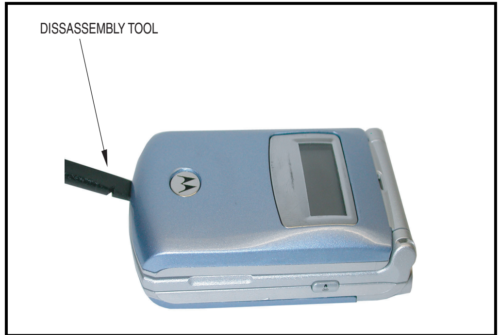
Figure 13. Removing the Flip Cover
