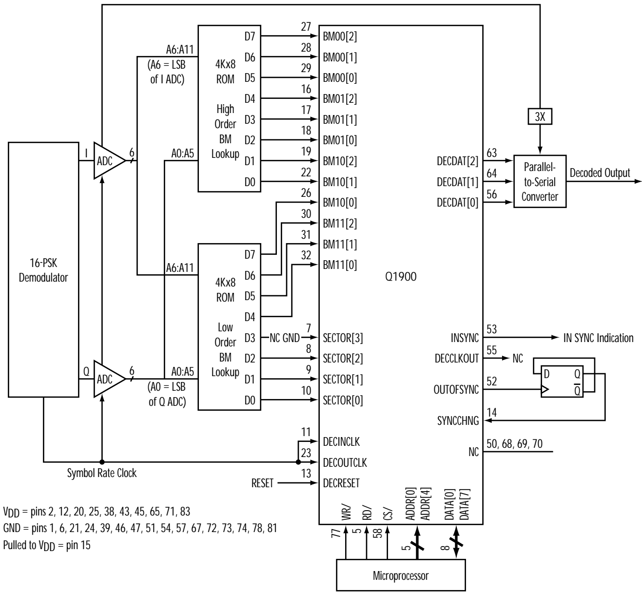
Figure 38. Rate \frac{3}{4} Trellis Mode Decoder Configuration Example for 84-pin PLCC* Package
