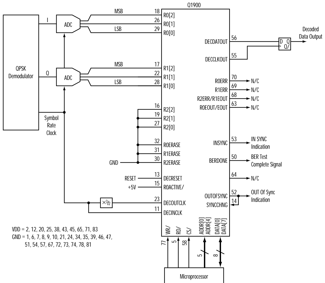
Figure 32. Rate \frac{3}{4} Parallel Viterbi Mode Decoder Example for 84-pin PLCC* Package
