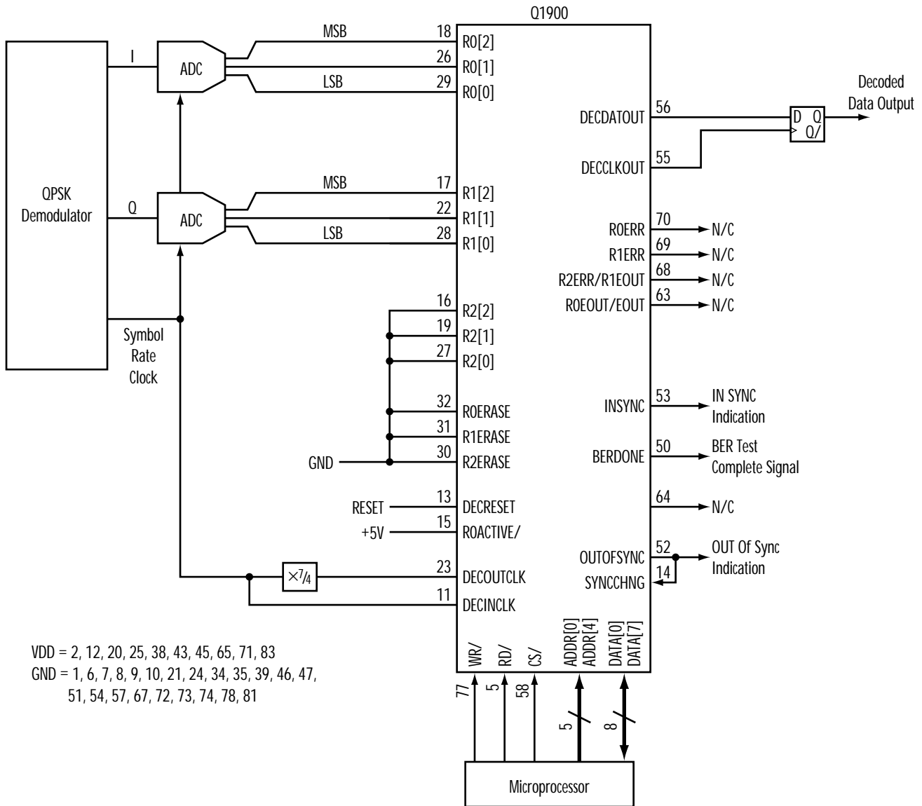
Figure 34. Rate \frac{7}{8} Parallel Viterbi Mode Decoder Example for 84-pin PLCC* Package
