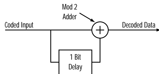
Figure 7. Differential Decoder
