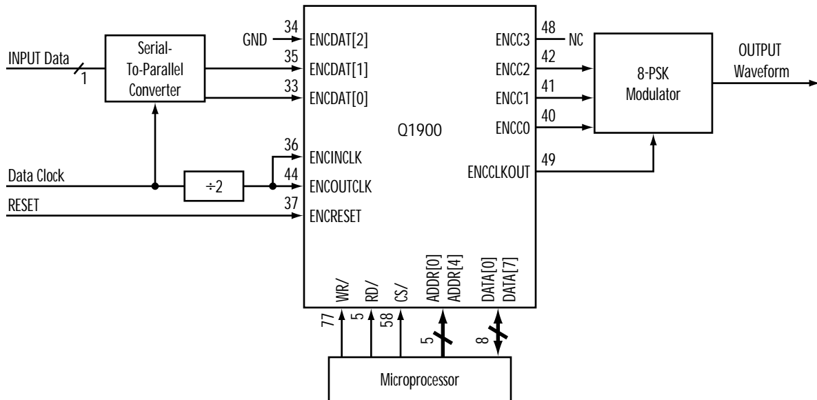
Figure 35. Rate 2/3 Trellis Mode Encoder Configuration Example for 84-pin PLCC* Package
