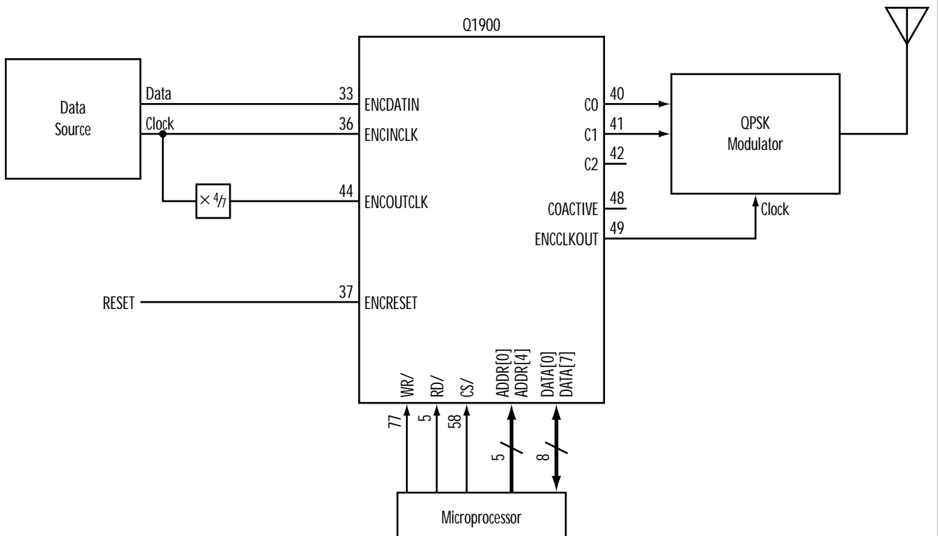
Figure 33. Rate \frac{7}{8} Parallel Viterbi Mode Encoder Example for 84-pin PLCC* Package
