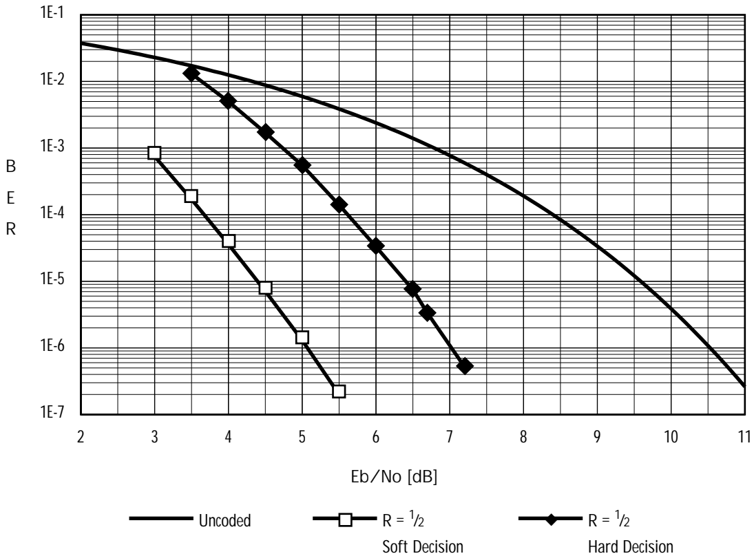
Figure 22. Hard Decision vs. Soft Decision Code Performance
