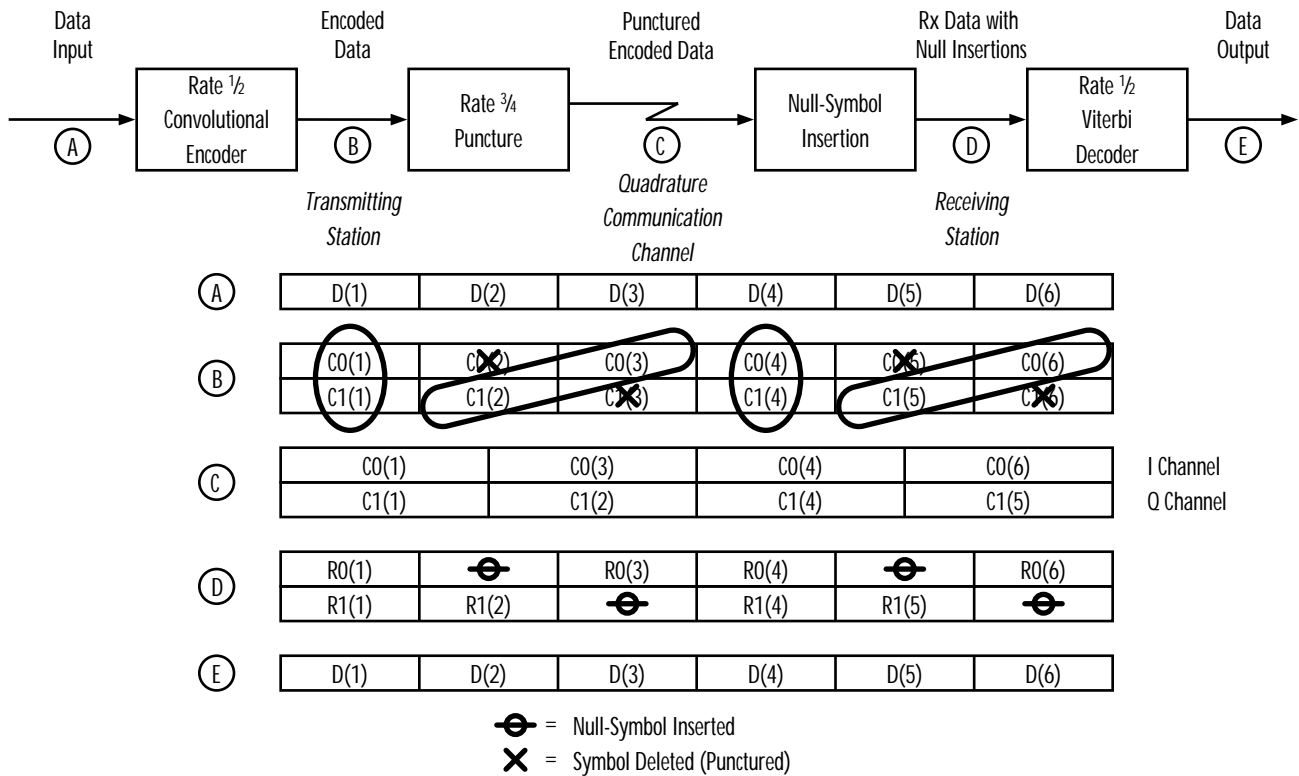
Figure 9a. Punctured Coding for Rate \frac{3}{4}
