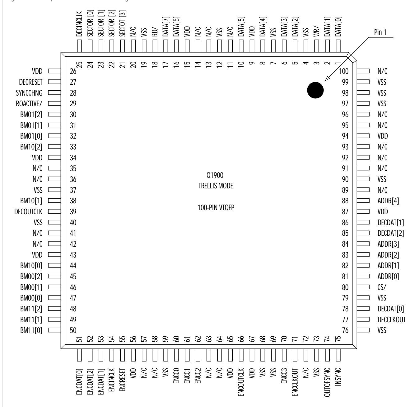
Figure 42. 100-pin Pinout for VTQFP Package for Trellis Mode
