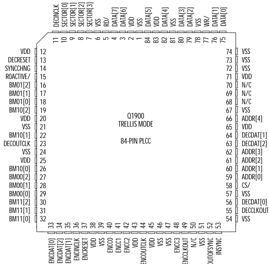
Figure 40. 84-pin Pinout for PLCC Packaging for Trellis Mode
