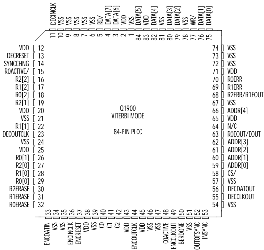
Figure 39. 84-PIN Pinout for PLCC Packaging for Viterbi Mode
