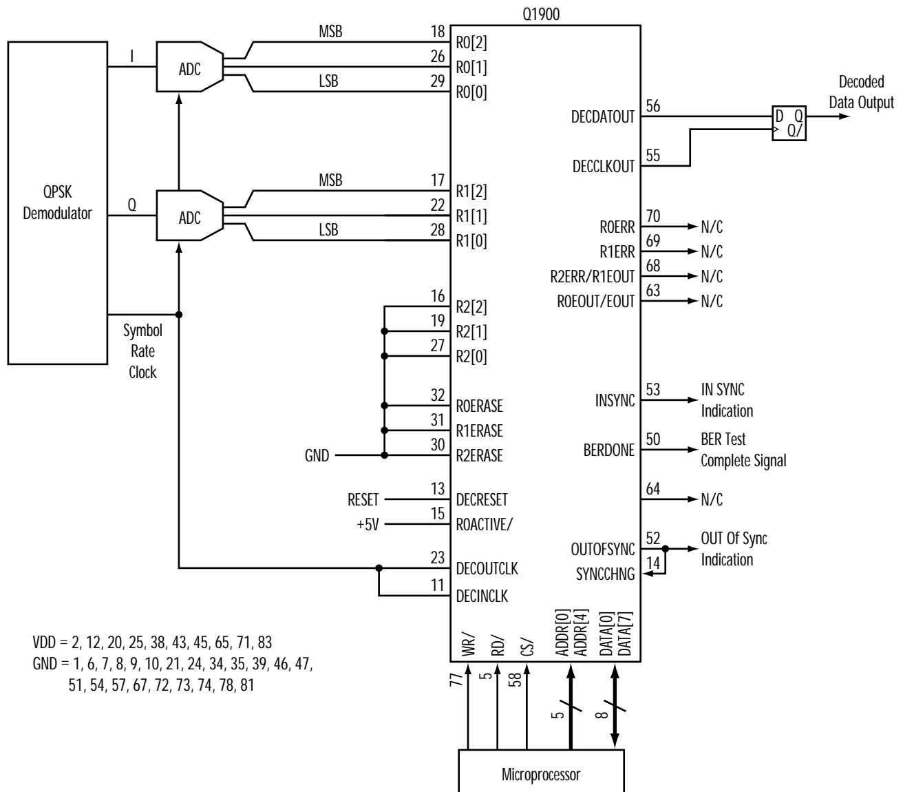
Figure 28. Rate 1/2 Parallel Viterbi Mode Decoder Example for 84-pin PLCC* Package
