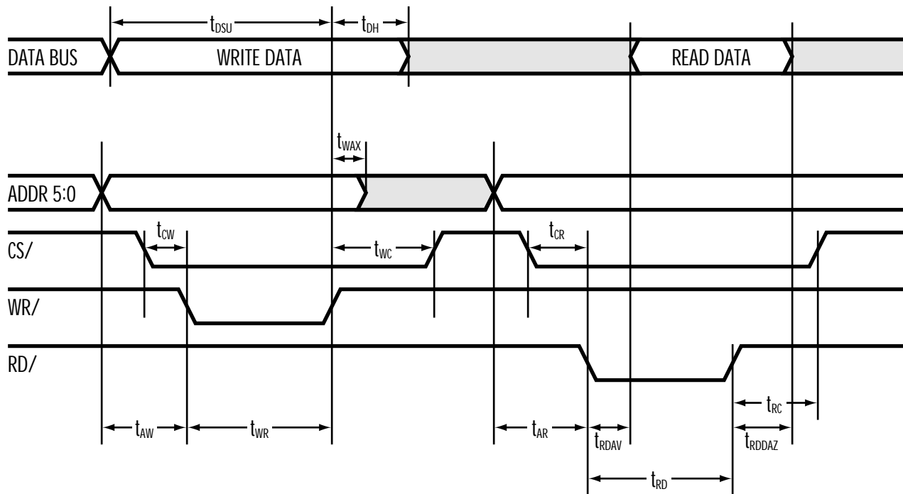
Figure 43. Processor Interface Timing Diagram
