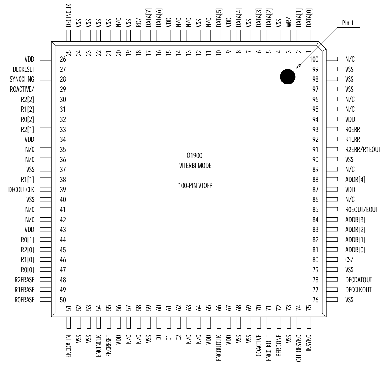
Figure 41. 100-PIN Pinout for VTQFP Packaging for Viterbi Mode
