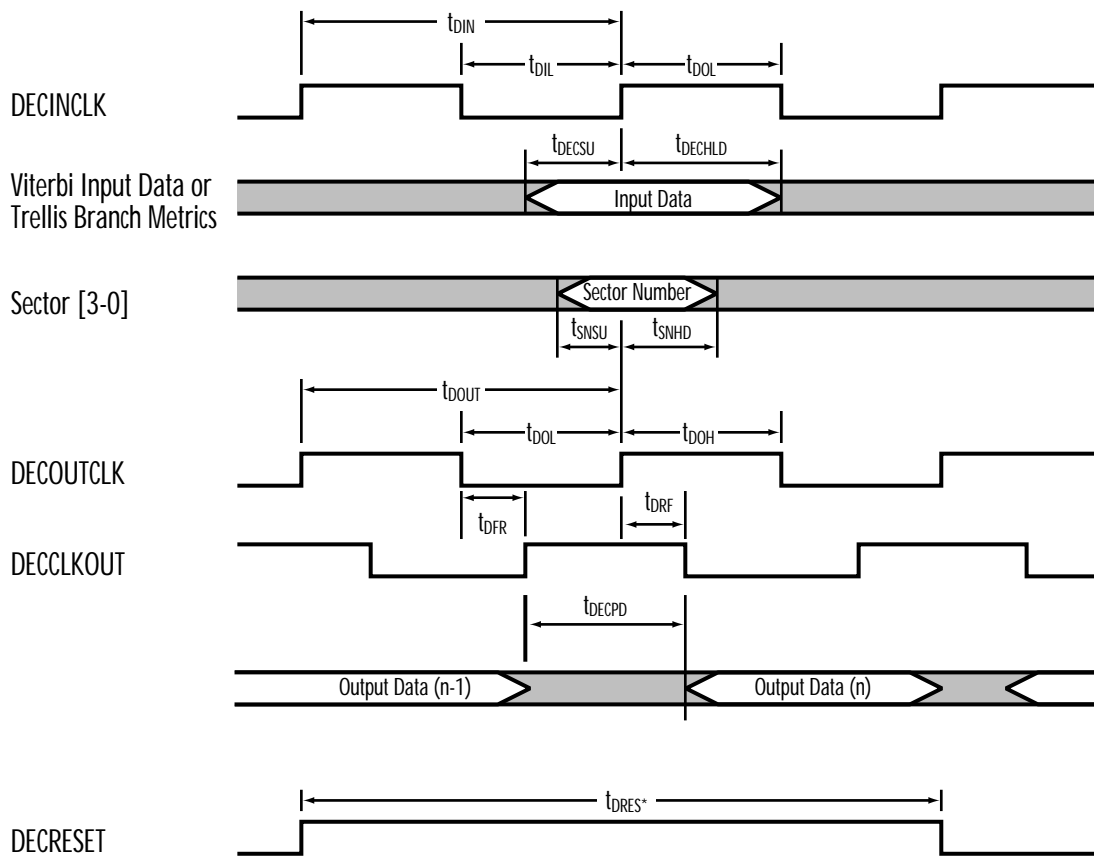
Figure 45. Decoder Clock Timing Diagram
