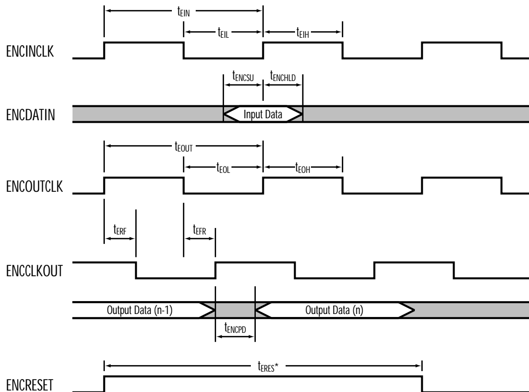
Figure 44. Encoder Clock Timing Diagram
