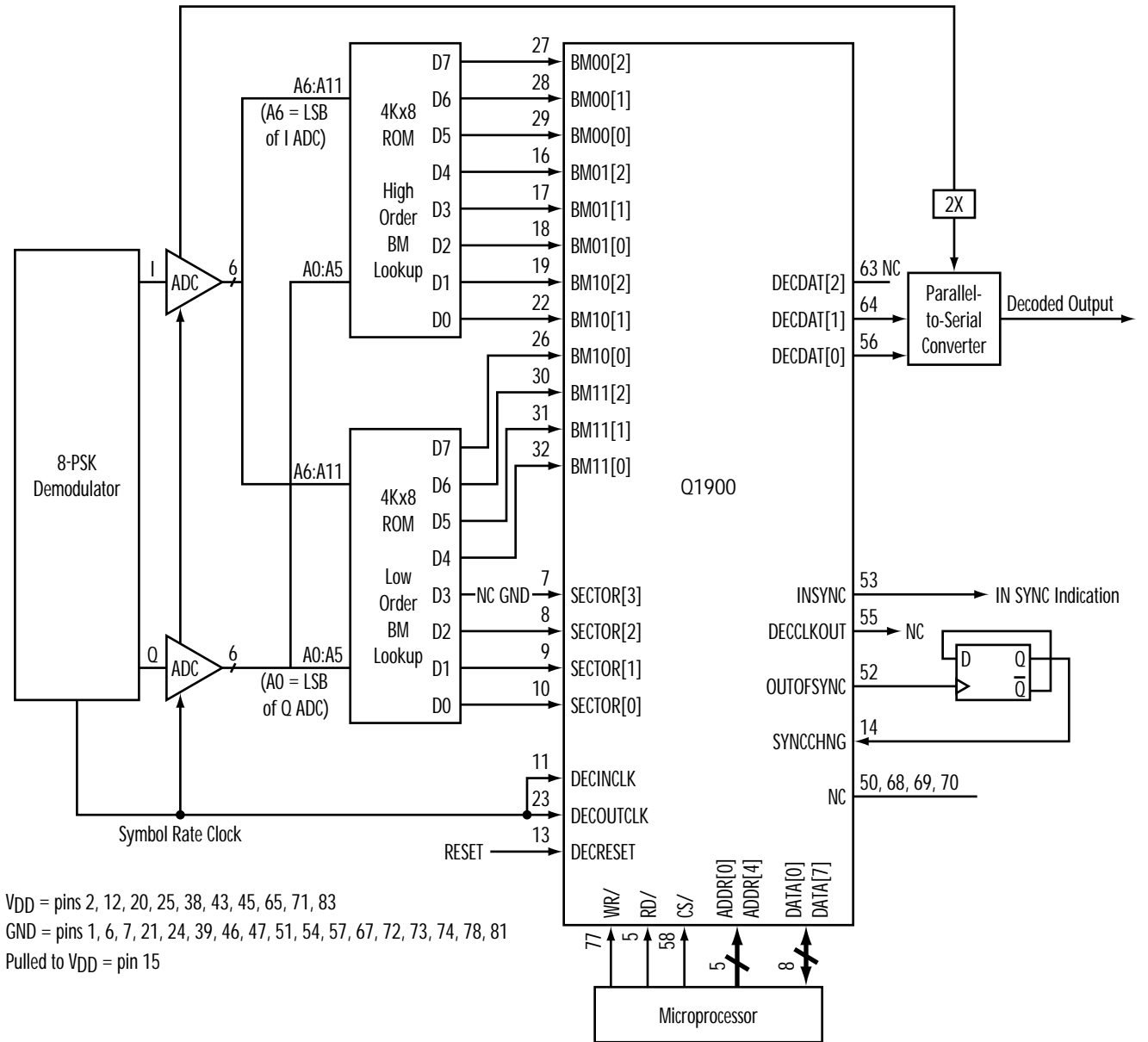
Figure 36. Rate 2/3 Trellis Mode Decoder Configuration Example for 84-pin PLCC* Package
