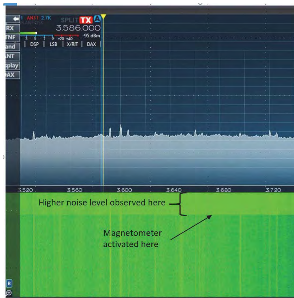
Figure 7. Noise observed on 80M.
