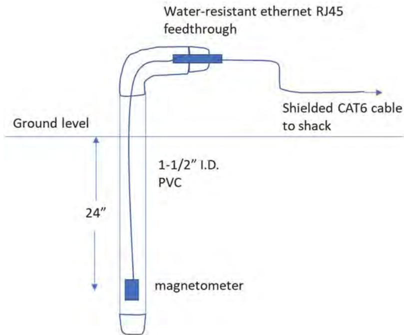
Figure 2. Magnetometer in-ground installation.
