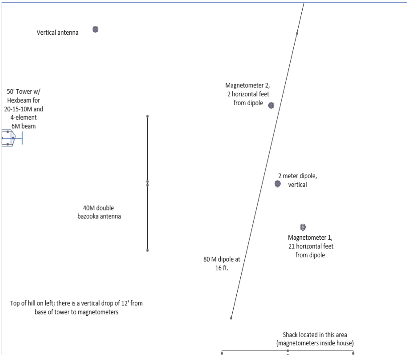
Figure 1. Layout of test area, showing antenna and magnetometer locations; approximately to scale.
