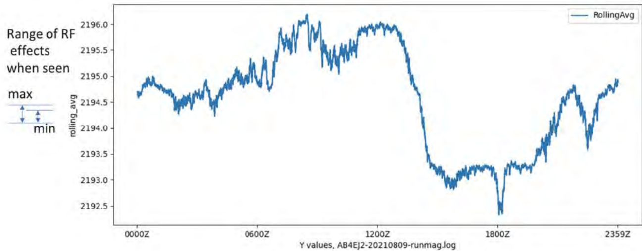
Figure 5. 24-hour plots of X and Y axes on magnetometer 2, with no RF exposure.
